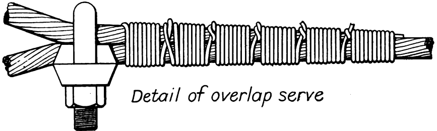
FIG. 136a.—Splicing messenger wire.
